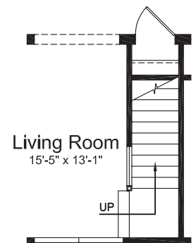
Optional Stairs at Living Room
